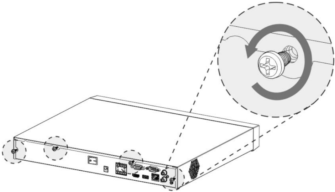
Figure 2-25 Remove cover
