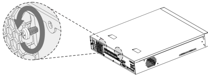
Figure 2-30 Remove screws
