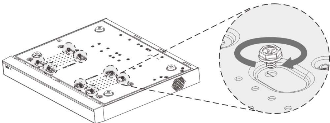
Figure 2-27 Fix HDD
