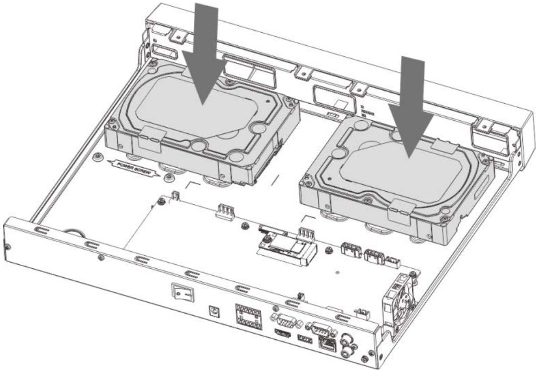
Figure 2-26 Place HDD
