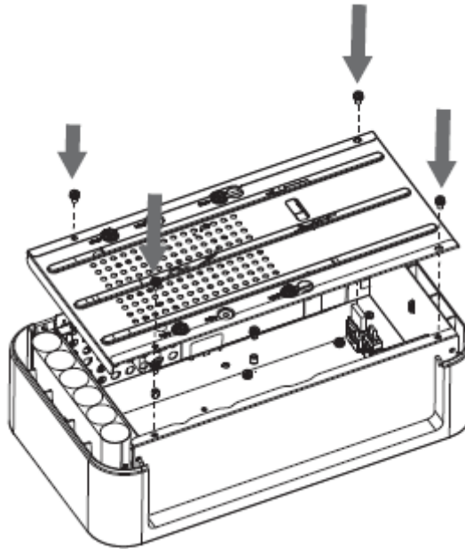
Figure 2-13 Fasten screws
