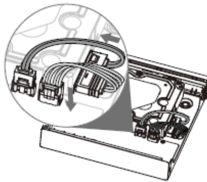
Figure 2-22 Connect cables
