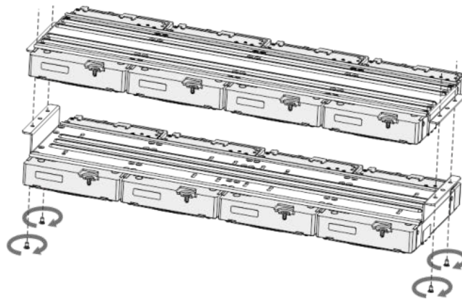
Figure 2-44 Put back drive bracket
