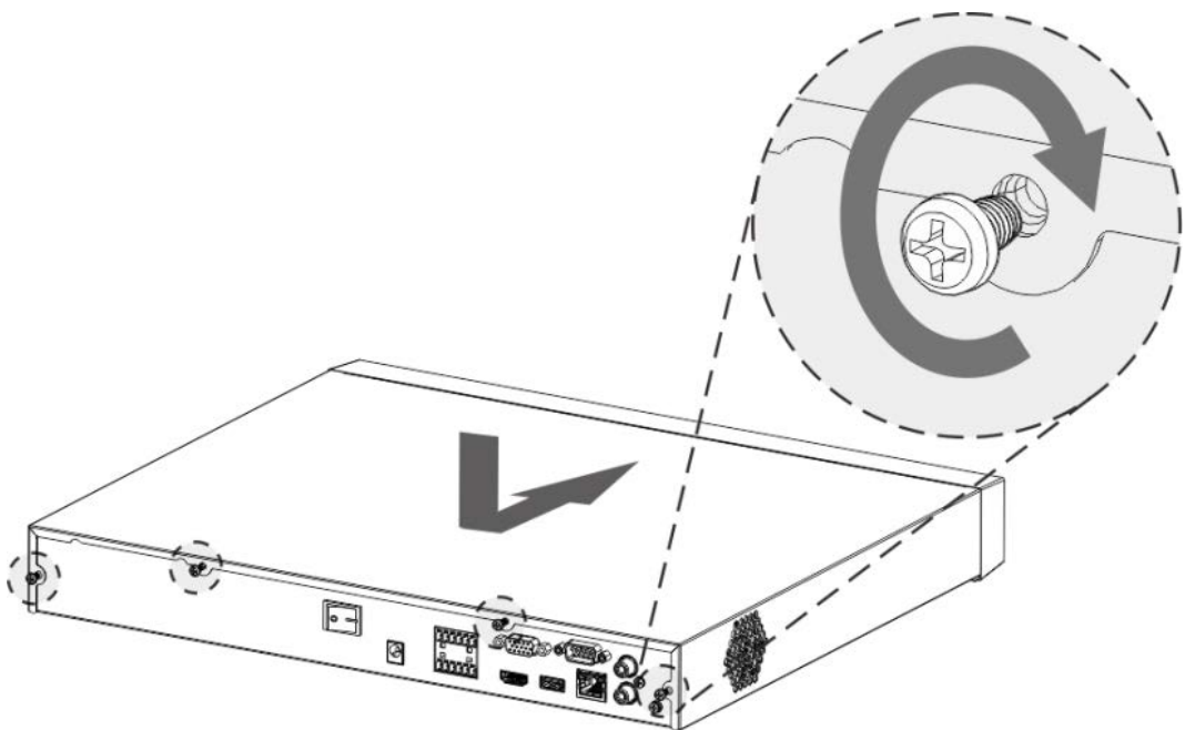
Figure 2-29 Fasten screws
