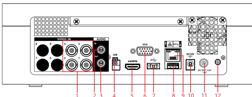
Figure 3-11 Rear panel (8-channel)
