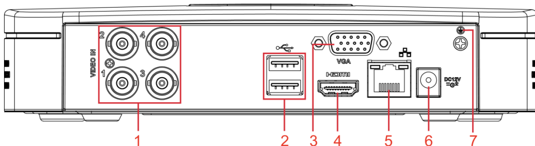
Figure 3-9 Rear panel
