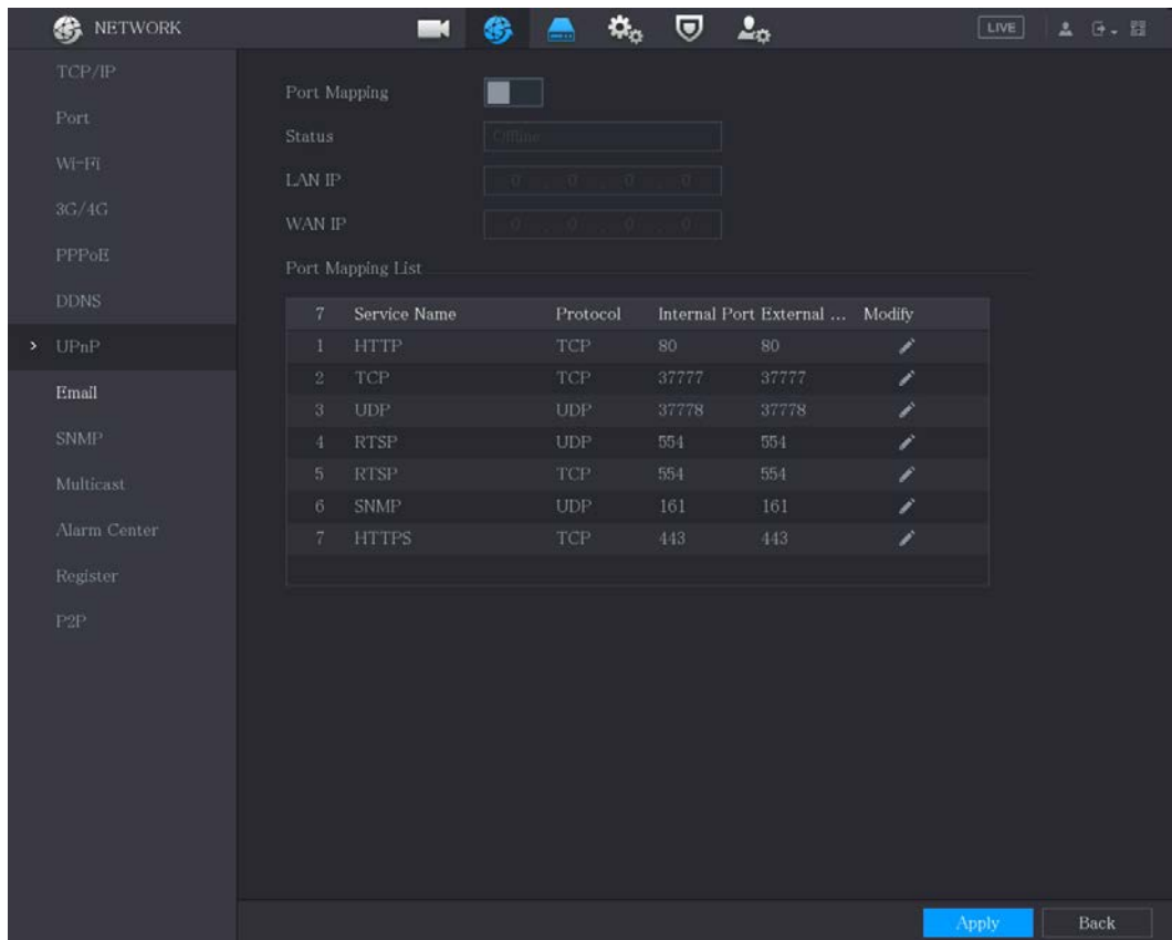
Figure 5-200 UPnP
